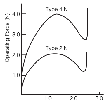
F-S Characteristics
