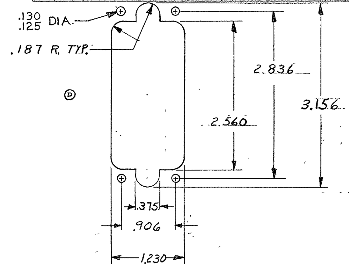
PANEL CUTOUT FULL SCALE
