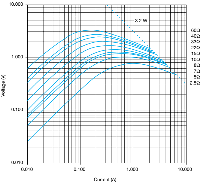
TYPICAL VOLTAGE/CURRENT CHARACTERISTICS FOR TYPE NF13
