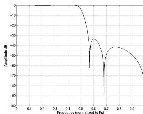
Figure 35. ADC Stopband Rejection
