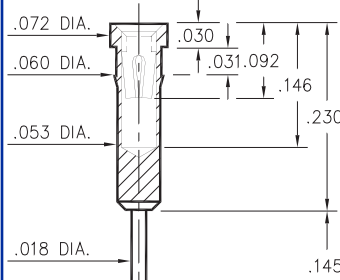
4001-0-15-XX-43-XX-04-0 Press-fit in .057 mounting hole
