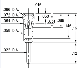
1023-0-15-XX-30-XX-04-0 Press-fit in .061 mounting hole
