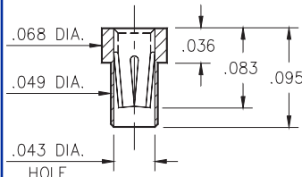
5342-0-15-XX-35-XX-10-0 Solder mount in .051 min. mounting hole
