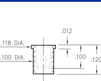
9372-0-15-XX-23-XX-10-0 Solder mount in .102 min. mounting hole
