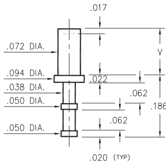
2305-X-00-XX-00-00-07-0 Swage mount in .076 hole
