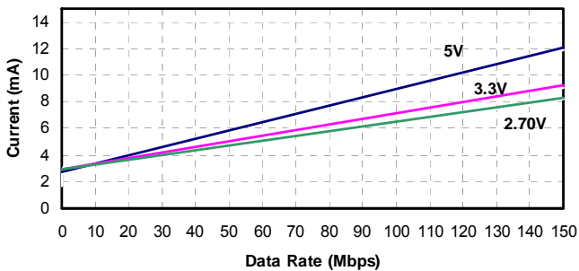
Figure 7. Si8441 Typical V_{DD1} Supply Current vs. Data Rate 5, 3.3, and 2.70 V Operation
