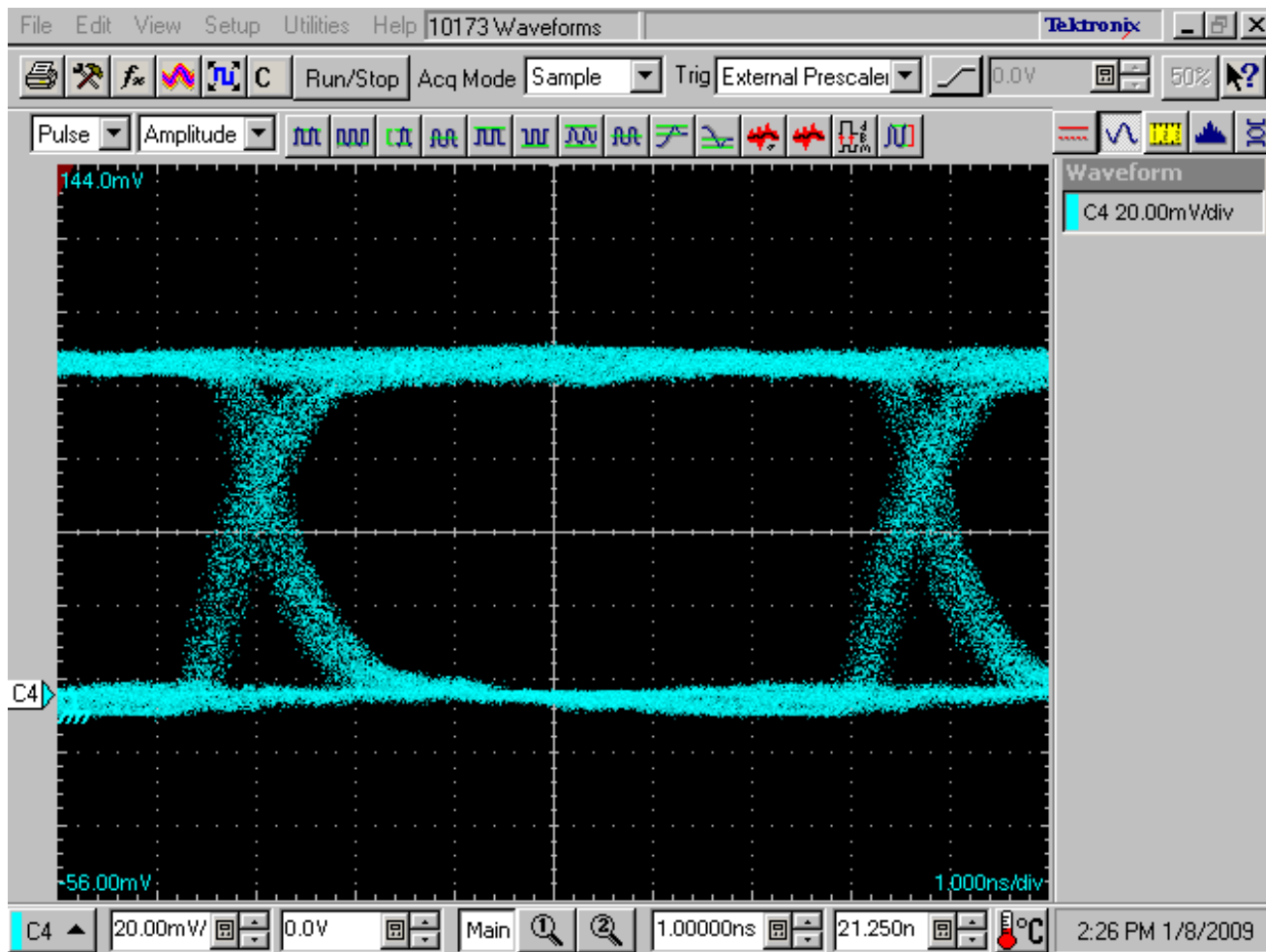
Figure 13. Eye Diagram
