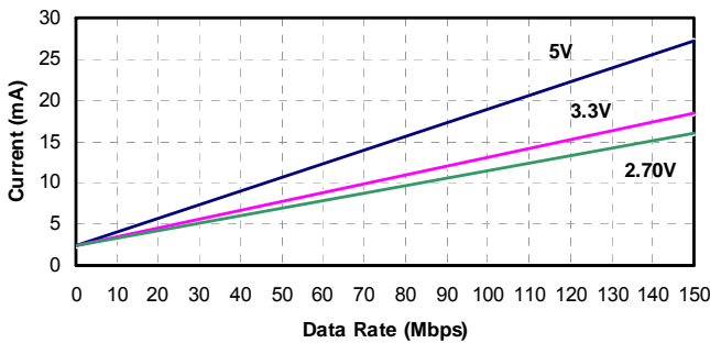
Figure 6. Si8440/45 Typical V_{DD2} Supply Current vs. Data Rate 5, 3.3, and 2.70 V Operation
