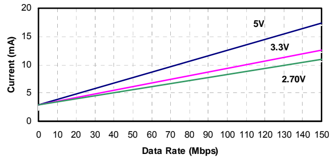
Figure 9. Si8442 Typical V_{DD1} or V_{DD2} Supply Current vs. Data Rate 5, 3.3, and 2.70 V Operation (15 pF Load)
