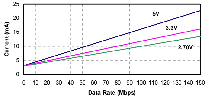
Figure 8. Si8441 Typical V_{DD2} Supply Current vs. Data Rate 5, 3.3, and 2.70 V Operation (15 pF Load)
