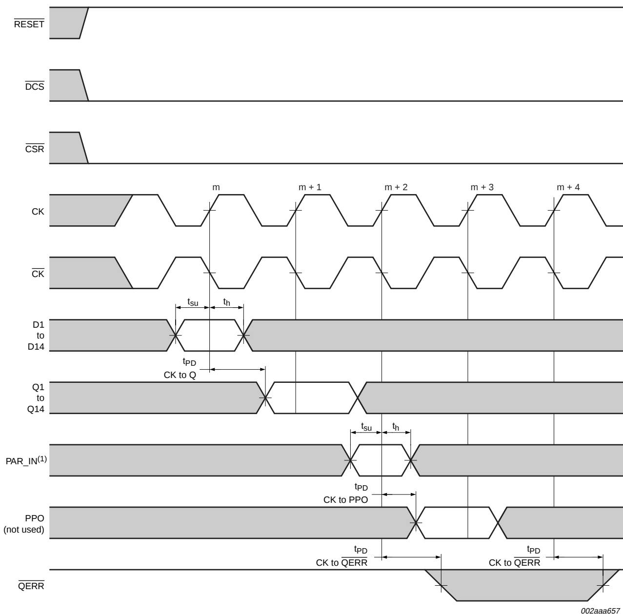
Fig 9. Timing diagram for the second SSTU32866 (1:2 Register B configuration) device used in pair; C0 = 1, C1 = 1
