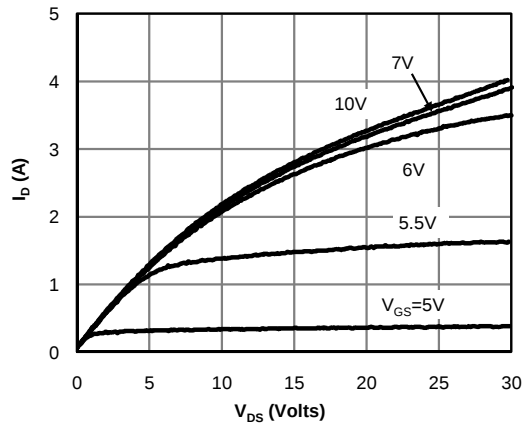
Fig 1: On-Region Characteristics
