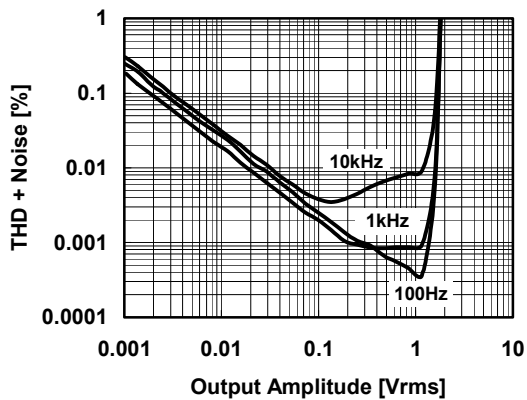
TOTAL HARMONIC DISTORTION + NOISE vs OUTPUT AMPLITUDE (Voltage Follower) NJM2737 , V^+/V^- = 2.5\text{V} , G_V=0\text{dB} R_L=2\text{k}\Omega , T_a=25^\circ\text{C}
