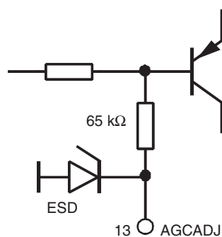
Figure 3-4. Internal Circuit at Pin AGCADJ
