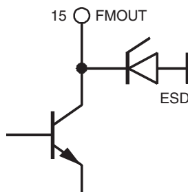
Figure 3-5. Internal Circuit at Pin FMOUT
