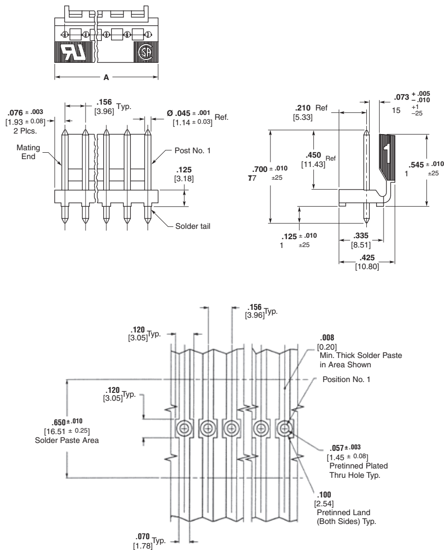
Recommended Mounting Hole Pattern for .062 [1.57] Thick PC Board
