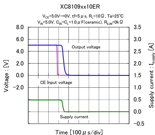
(21) Turn-off delay vs. Fall time ( C_L=1.0\ \mu\text{F} )
