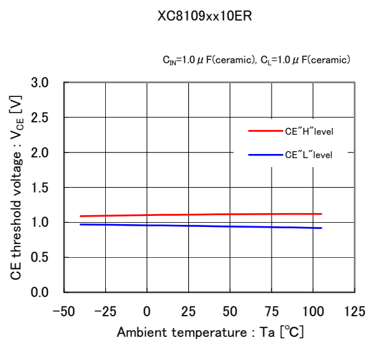
(10) CE threshold voltage vs. Ambient temperature
