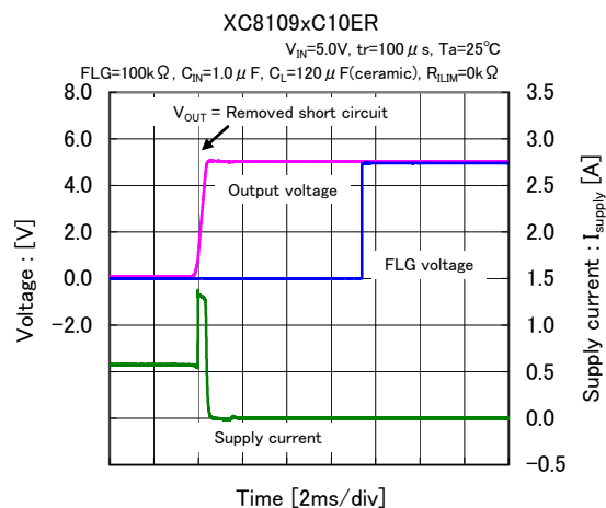
(32) Short-circuit transient response
