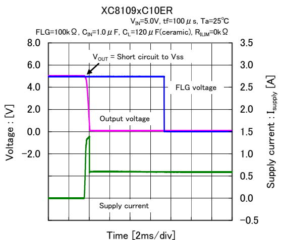
(31) Short-circuit transient response
