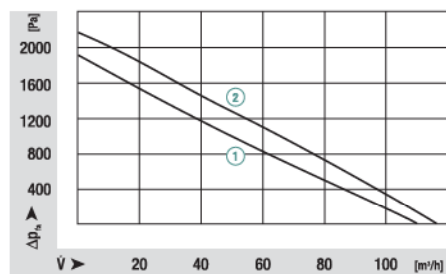
Characteristic curves
