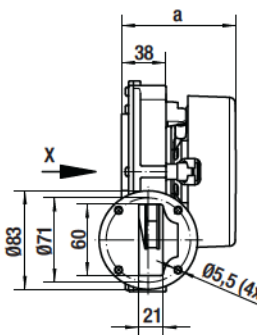
view X Honeywell flange on request
