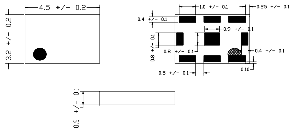
[MECHANICAL DIMENSIONS]
