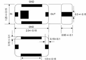
[MECHANICAL DIMENSIONS]
