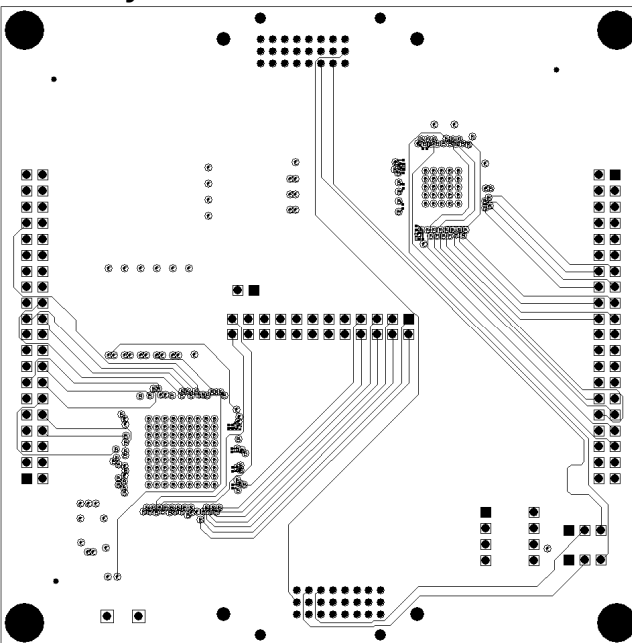
Bottom Board
