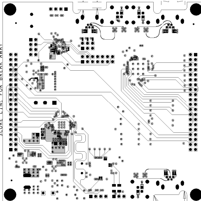
Top Board
