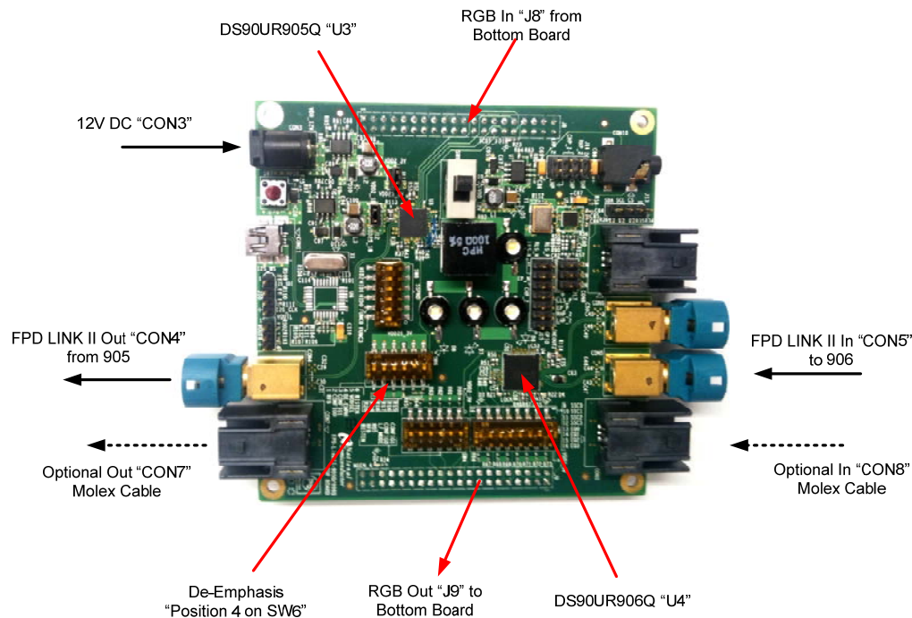
Figure 4. Top Board
