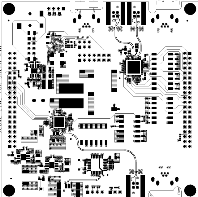
Top Board
