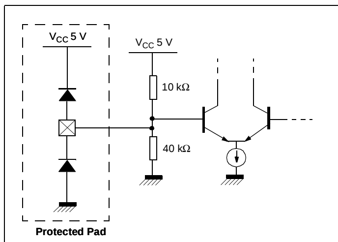
Figure 15: DECV (Pin 5)
