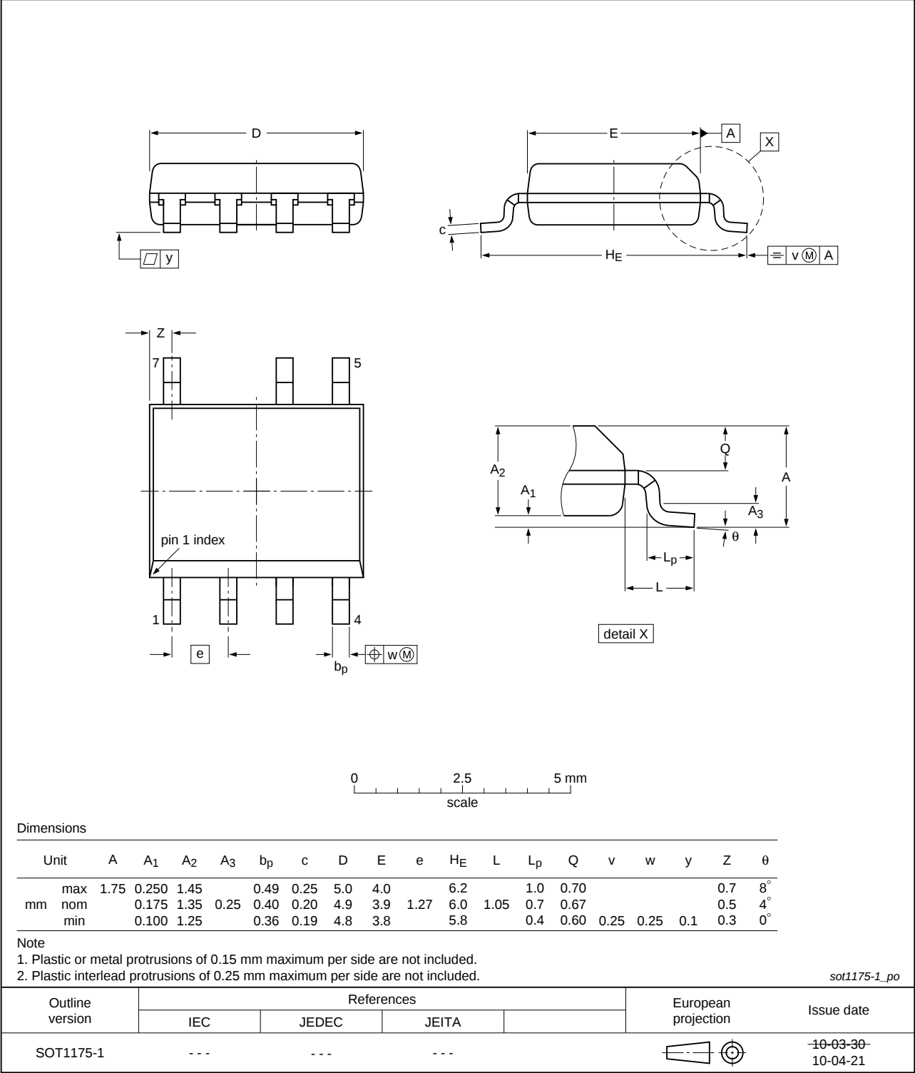
Fig 5. Package outline SOT1175-1 (SOT7)
