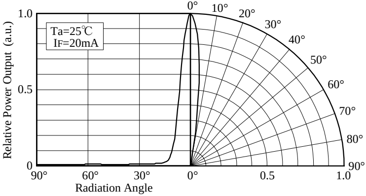
■ Directivity (NSHU590A)
