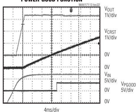
POWER-GOOD FUNCTION
