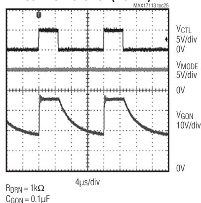
HIGH-VOLTAGE SWITCH CONTROL FUNCTION (MODE 1)
