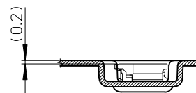
SECTION X-X
