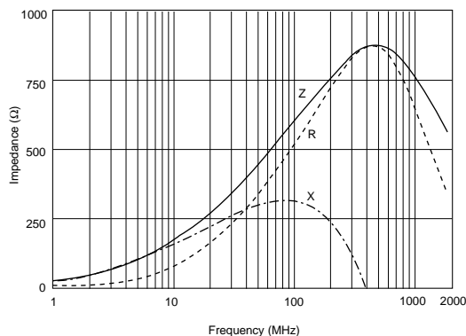
BLM18HG601SH1
