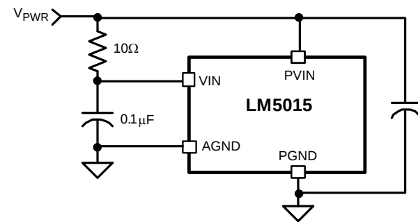
(a) Analog Input Powered from the Main Power
