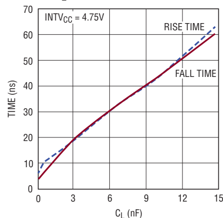
Gate Driver Rise and Fall Time vs C L
