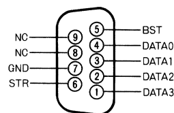
D-sub Connector Output
