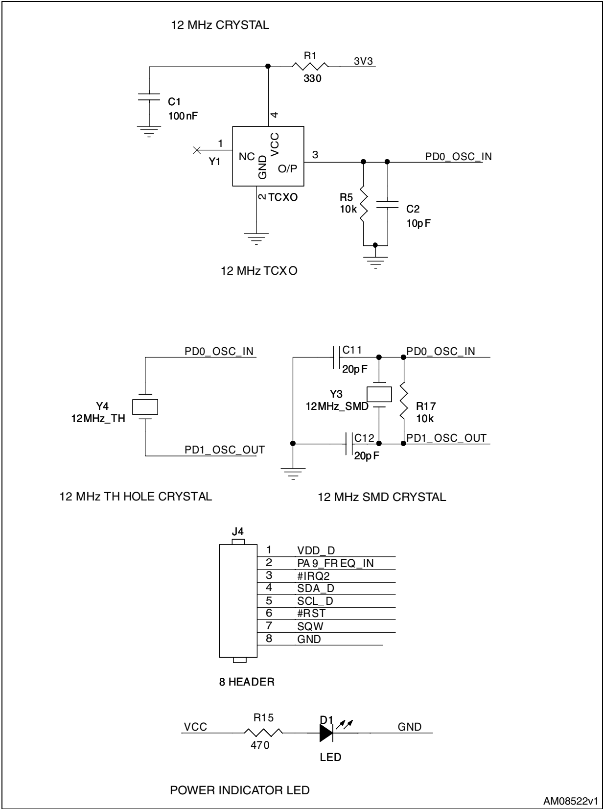
Figure 5. Schematic 5 of 5
