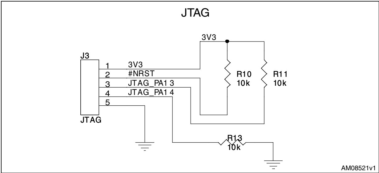
Figure 4. Schematic 4 of 5
