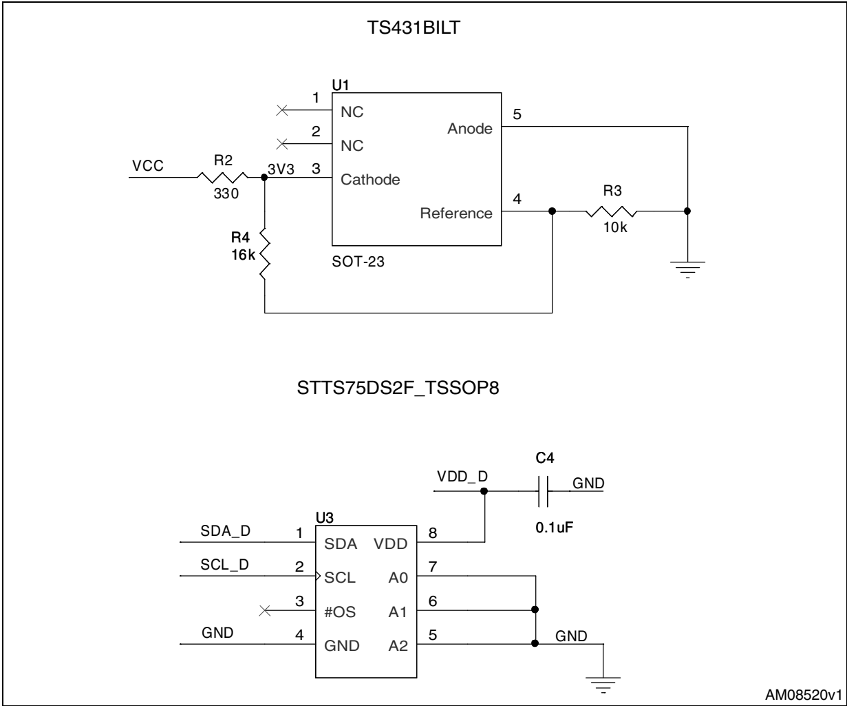
Figure 3. Schematic 3 of 5
