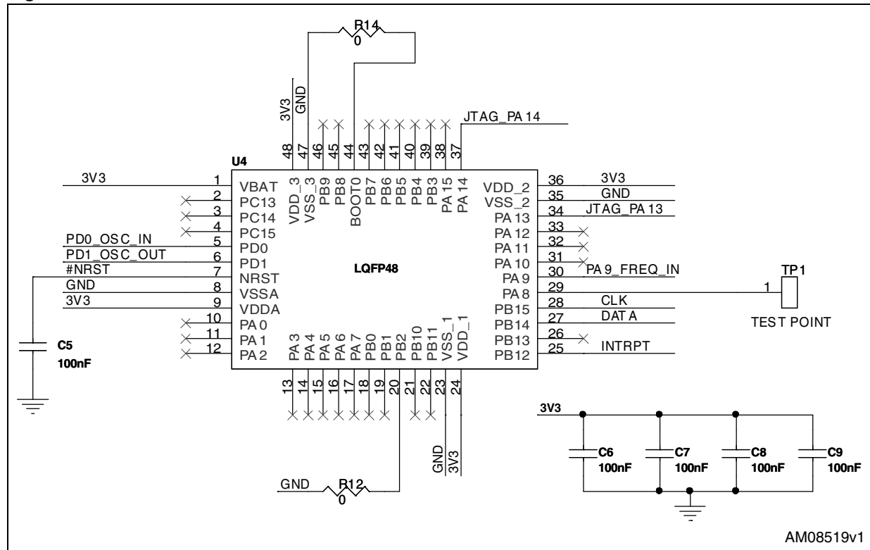
Figure 2. Schematic 2 of 5
