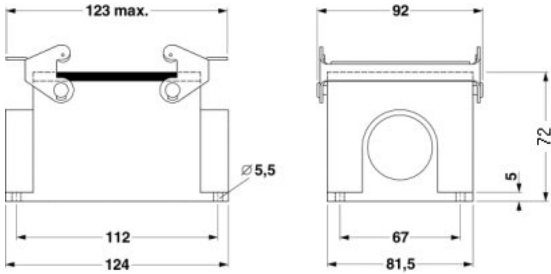
Dimensioned drawing
