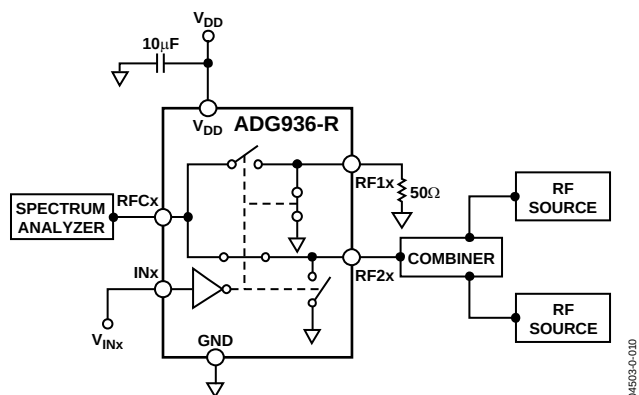
Figure 25. IP_3
