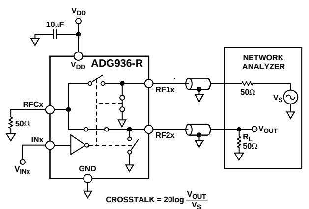
Figure 23. Crosstalk
