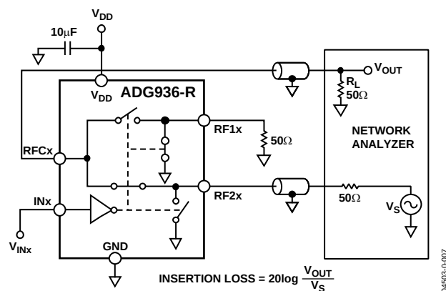
Figure 22. Insertion Loss
