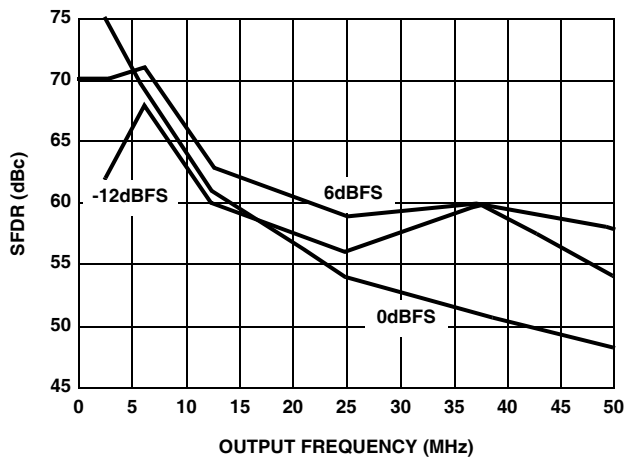
FIGURE 5. SFDR vs f_{OUT} , CLOCK = 125MSPS
