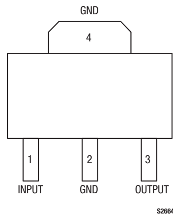
Figure 2. SKY65016-70LF Pinout – 4-Pin SOT-89 Package (Top View)
