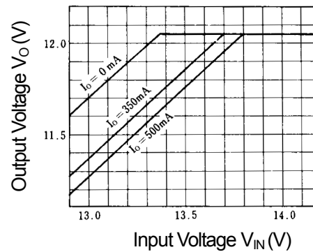
NJM78M12 Dropout Characteristics
