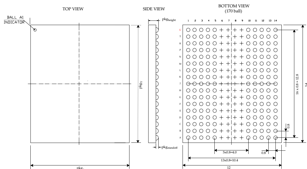
Figure 84. Package Dimensions
