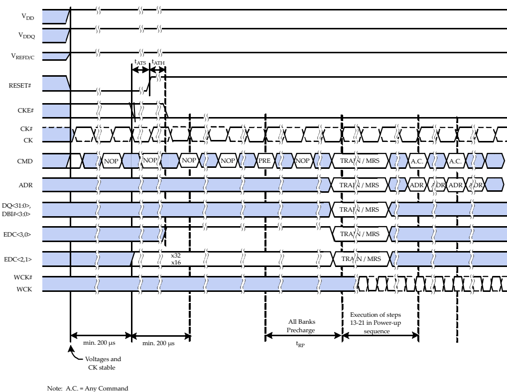
Figure 3: GDDR5 SGRAM Power-up Initialization
