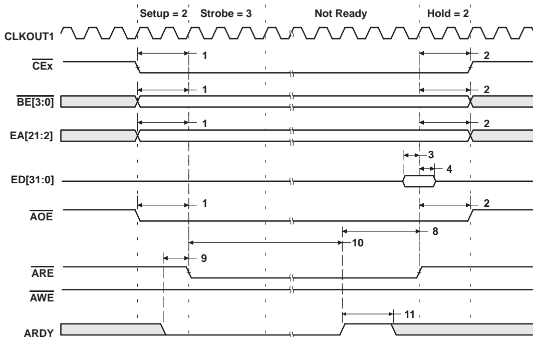
Figure 18. Asynchronous Memory Read Timing (ARDY Used)
