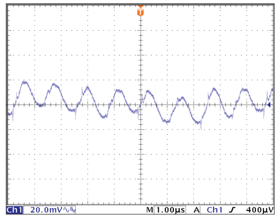
Power-On Startup (V IN = 12 V, I OUT = 25 A)
