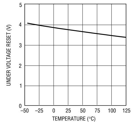
Undervoltage Reset Voltage vs Temperature
