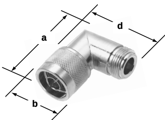
N Angle Adapters, Plug-Jack 82-64
