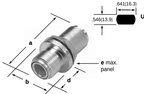
Jack to Jack Bulkhead Adapter 82-66
