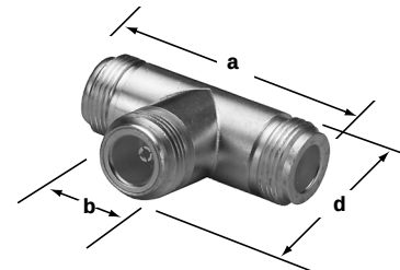
N Tee Adapter Jack-Jack-Jack 82-99
