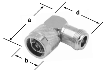
N Angle Adapter, Plug-Jack 82-213 82-64-RFX
