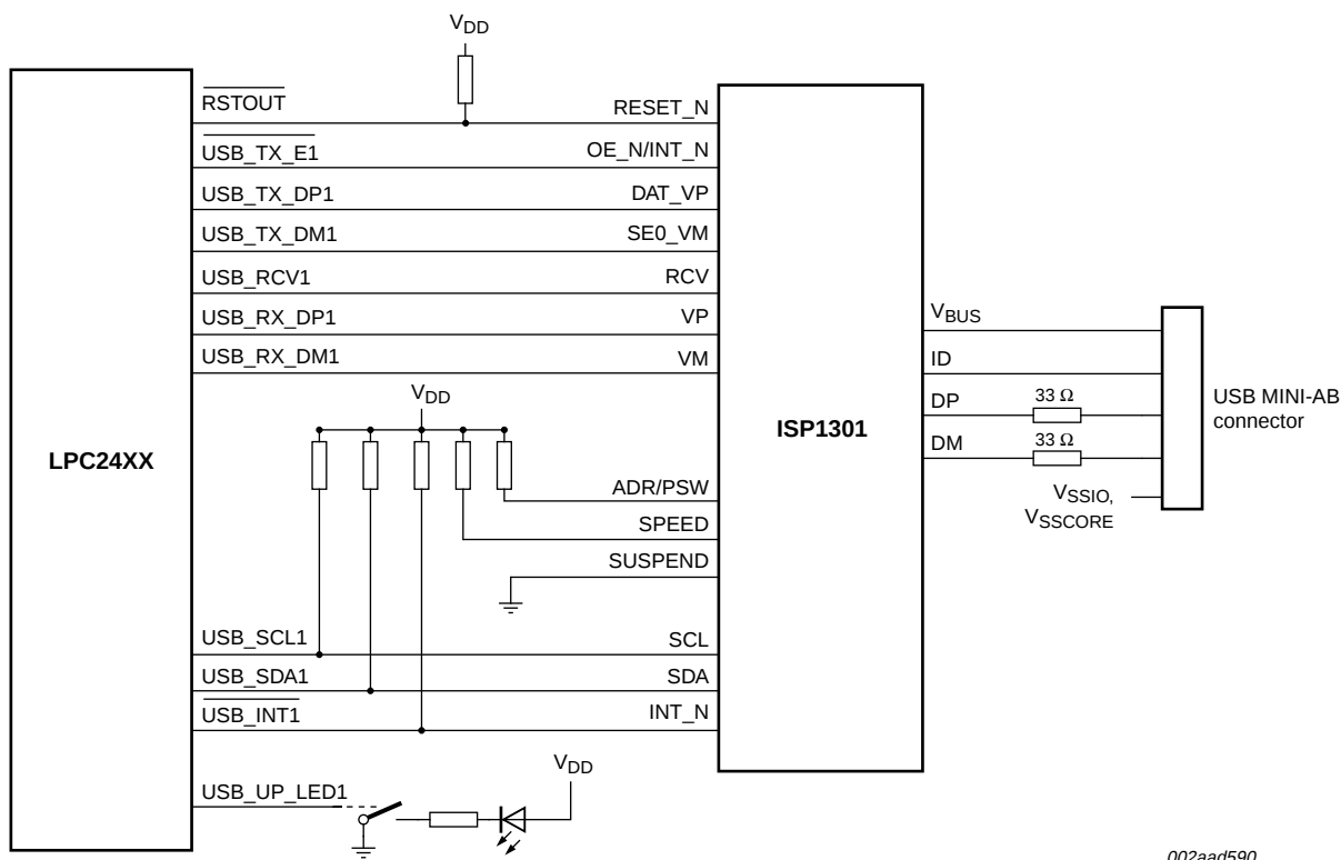
Fig 15. LPC2458 USB OTG port configuration: VP_VM mode
