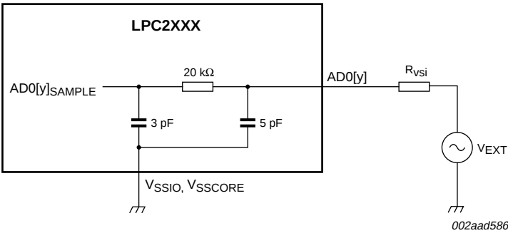
Fig 5. Suggested ADC interface - LPC2458 AD0[y] pin
