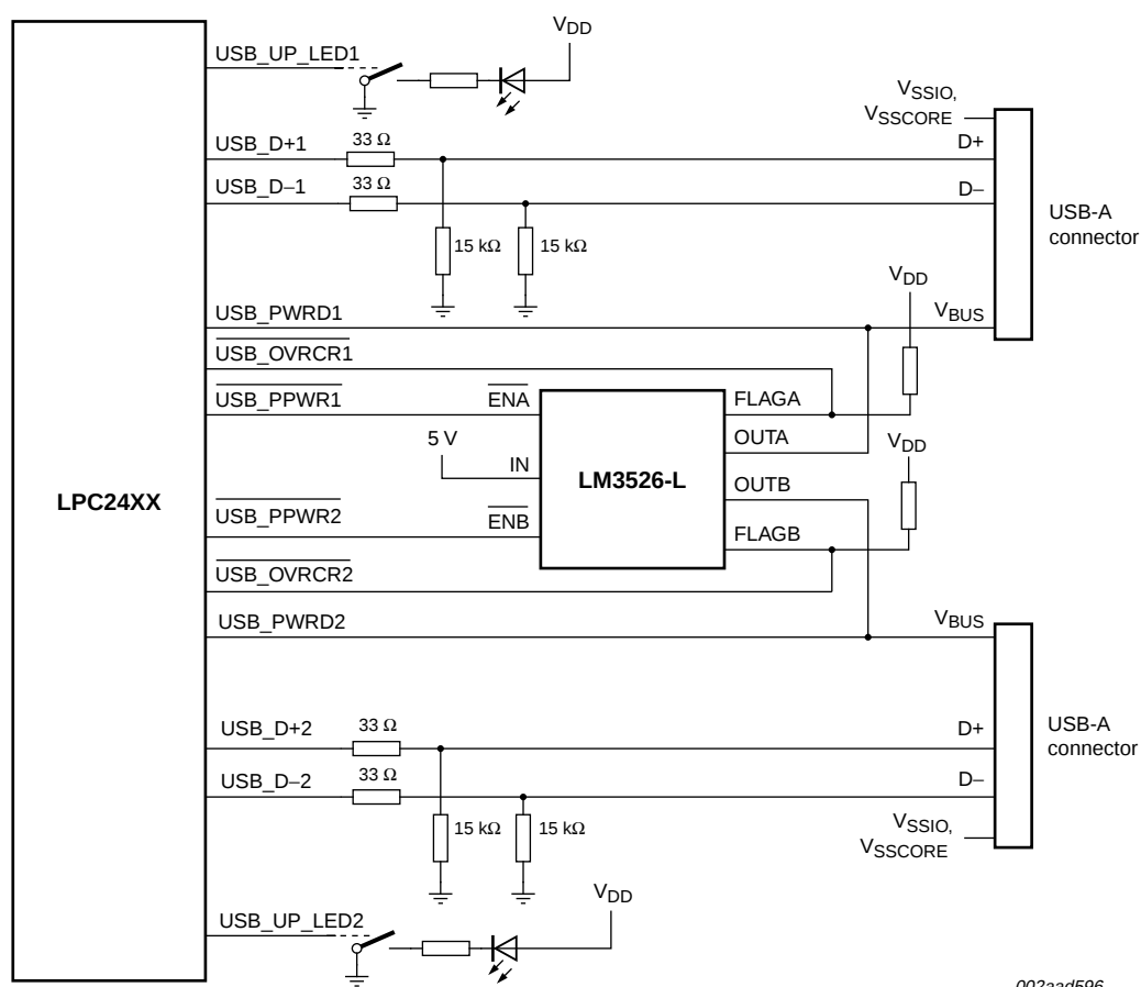
Fig 17. LPC2458 USB OTG port configuration: USB port 1 host, USB port 2 host
