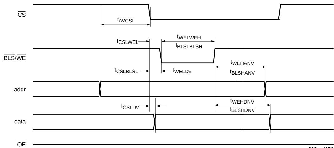
Fig 10. External memory write access
