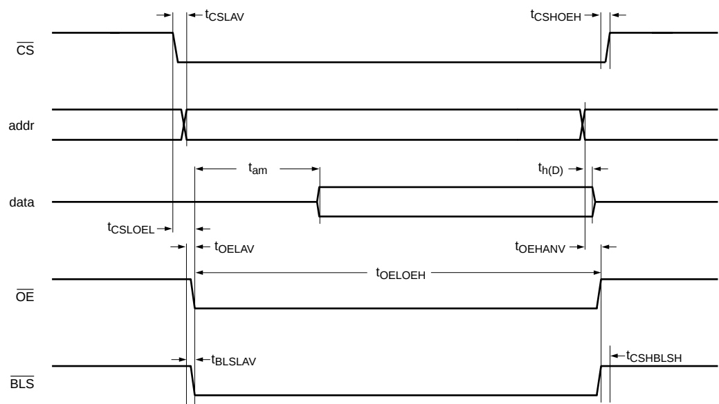
Fig 9. External memory read access
