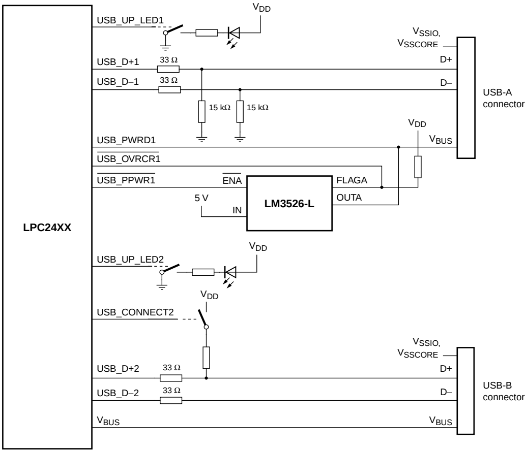
Fig 16. LPC2458 USB OTG port configuration: USB port 2 device, USB port 1 host
