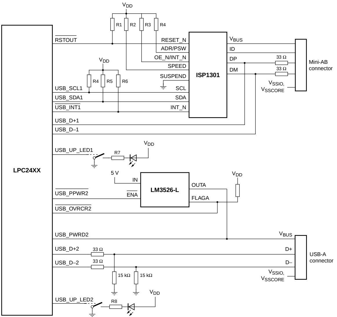
Fig 14. LPC2458 USB OTG port configuration: USB port 1 OTG dual-role device, USB port 2 host
