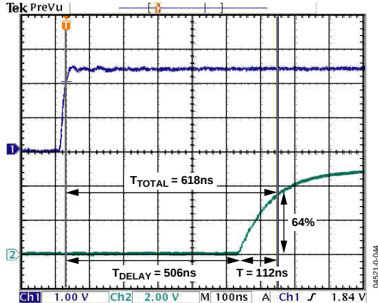
Figure 20. OrFET Turn-On Time (Inverse Polarity)
