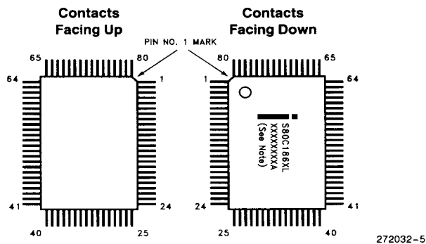
Figure 2. 80C186XL Pinout Diagrams (Continued)
