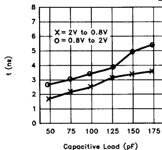
Typical Rise and Fall Times for TTL Voltage Levels
