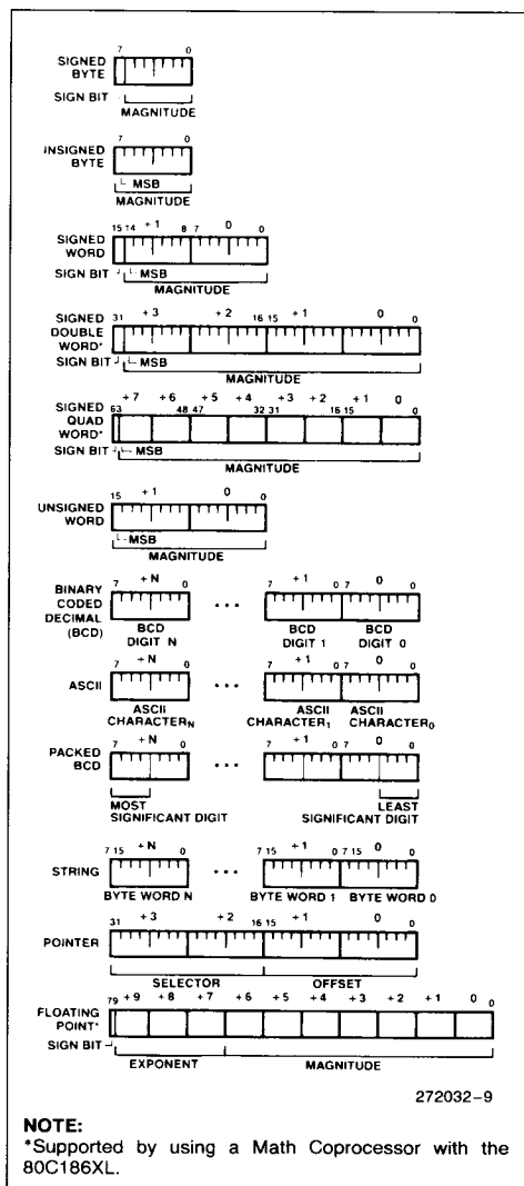
Figure 7. 80C186XL Supported Data Types
