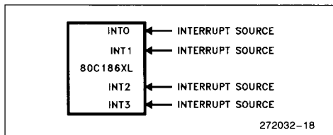
Figure 22. Fully Nested (Direct) Mode Interrupt Controller Connections
