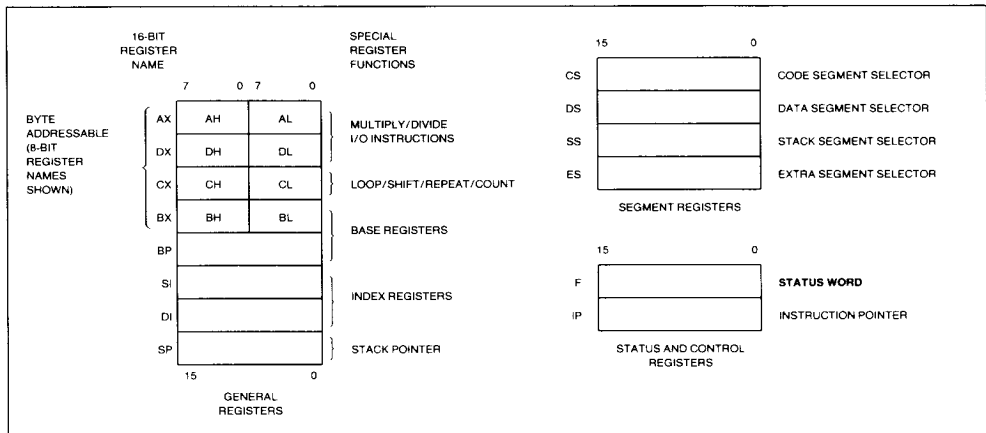
Figure 3a. 80C186XL Register Set
