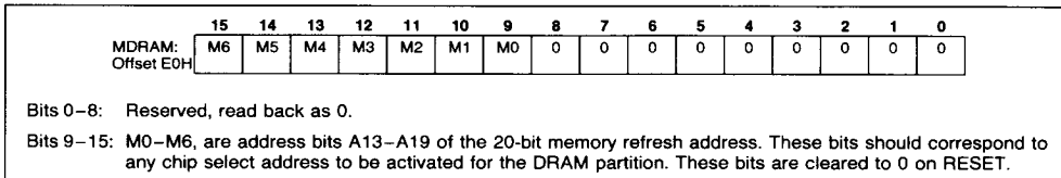
Figure 40. Memory Partition Register
