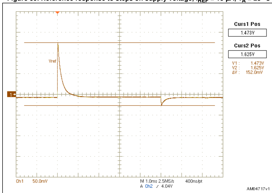
Figure 39. Reference response to steps on supply voltage, I_{REF} = 15\ \mu\text{A} , T_A = 25\ ^\circ\text{C}
