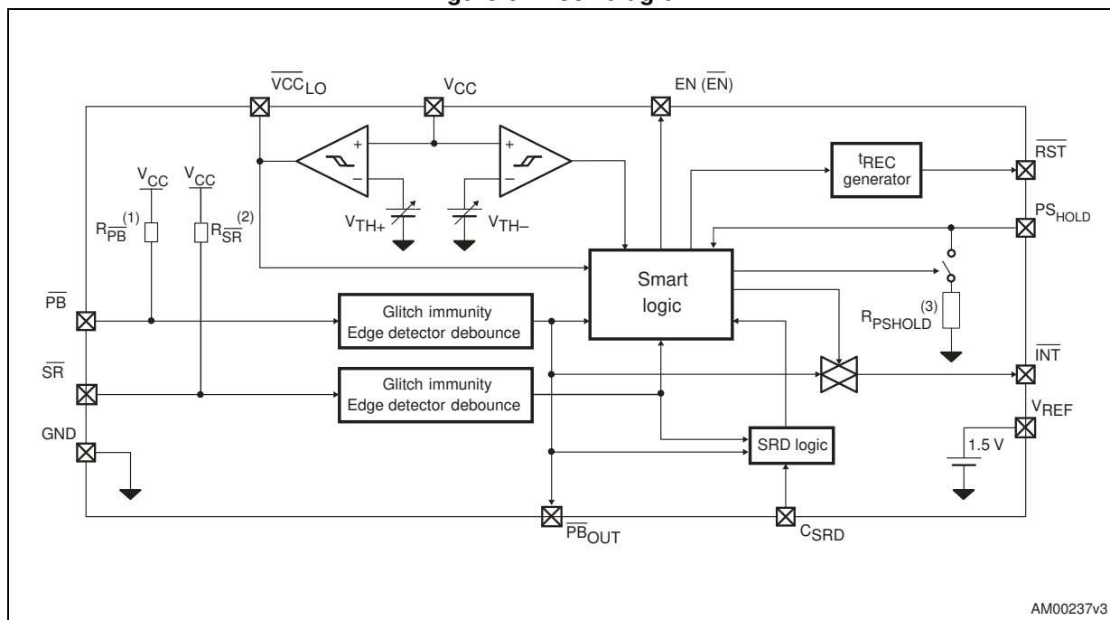
Figure 6. Block diagram
