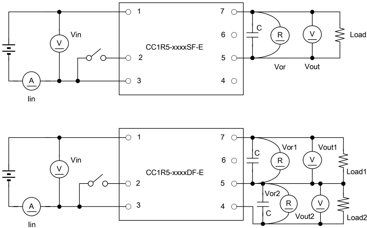
[5] Test Circuit
