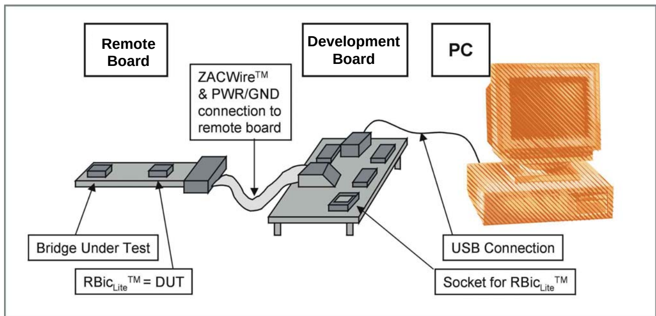
Figure 1.1 – RBic dLite TM Development Kit
