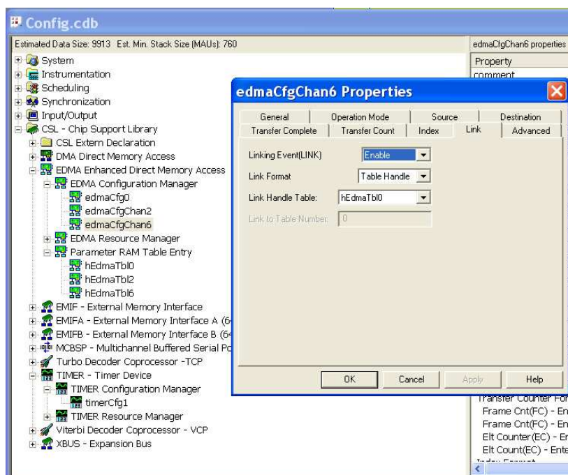
Figure 3. Screenshot of DSP/BIOS Configuration File
