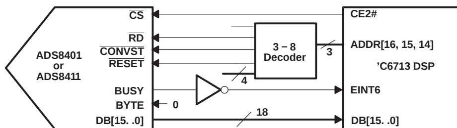
Figure 1. Hardware Connection
