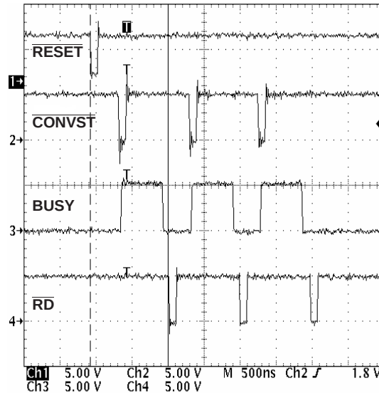
Figure 4. Scope Screenshot Showing Power-on Initialization Cycles
