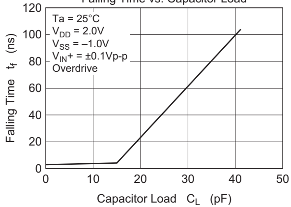
Figure 4-15 HA1631S04 Falling Time, t_f (Overdrive = \pm 0.1\text{Vp-p} )
