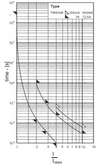
Time-Current Characteristics
