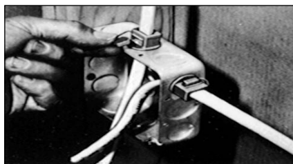
Snap captive locking wedge into connector's cavity.
