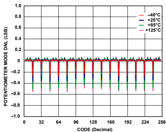
Figure 6. DNL vs. Code, V_{DD} = 5\text{ V}
