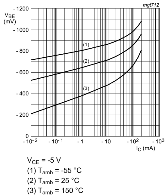
Fig. 3. BC857AW: Base-emitter voltage as a function of collector current; typical values
