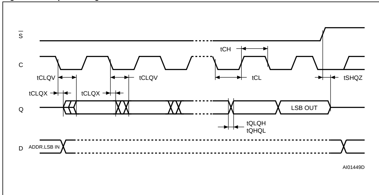
Figure 24. Output Timing
