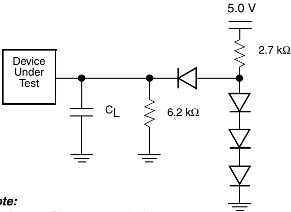
Figure 9. Test Setup
