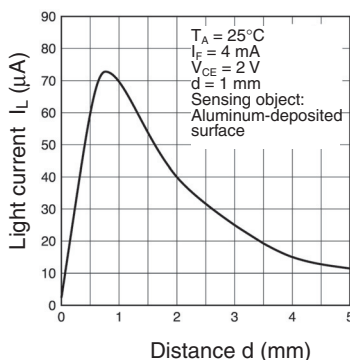
Sensing Distance Characteristics (Typical)
